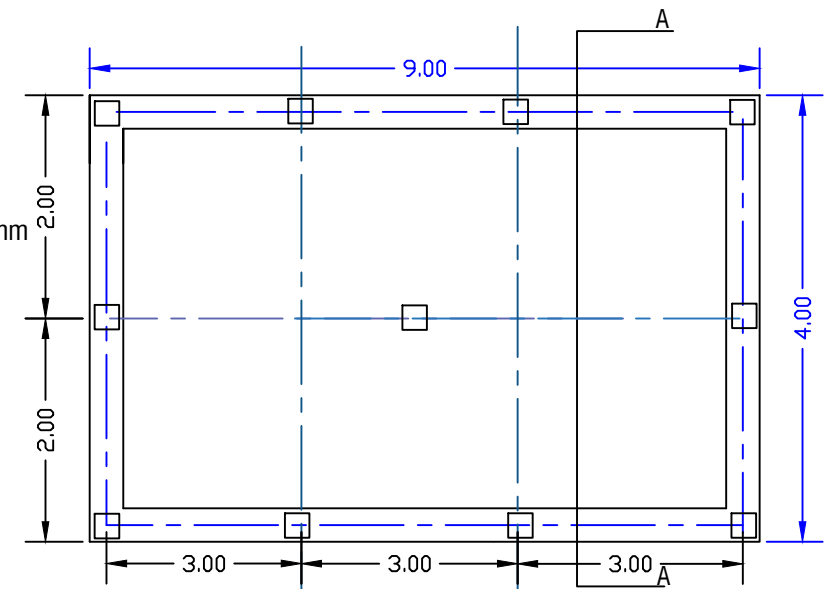
Plan elevation
